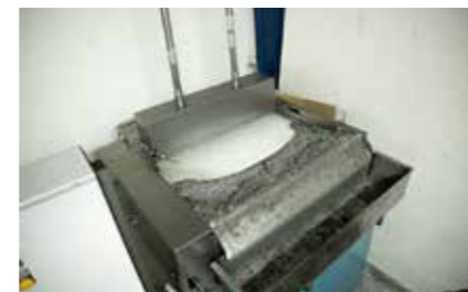
Hydrostatic band filter for filtering particles and metal chips from the coolant.
